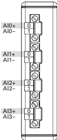
Figure 2. NI 9227 Terminal Assignments
